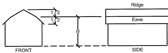
FIGURE 2-1: Interpretation of Building Height Measurement
