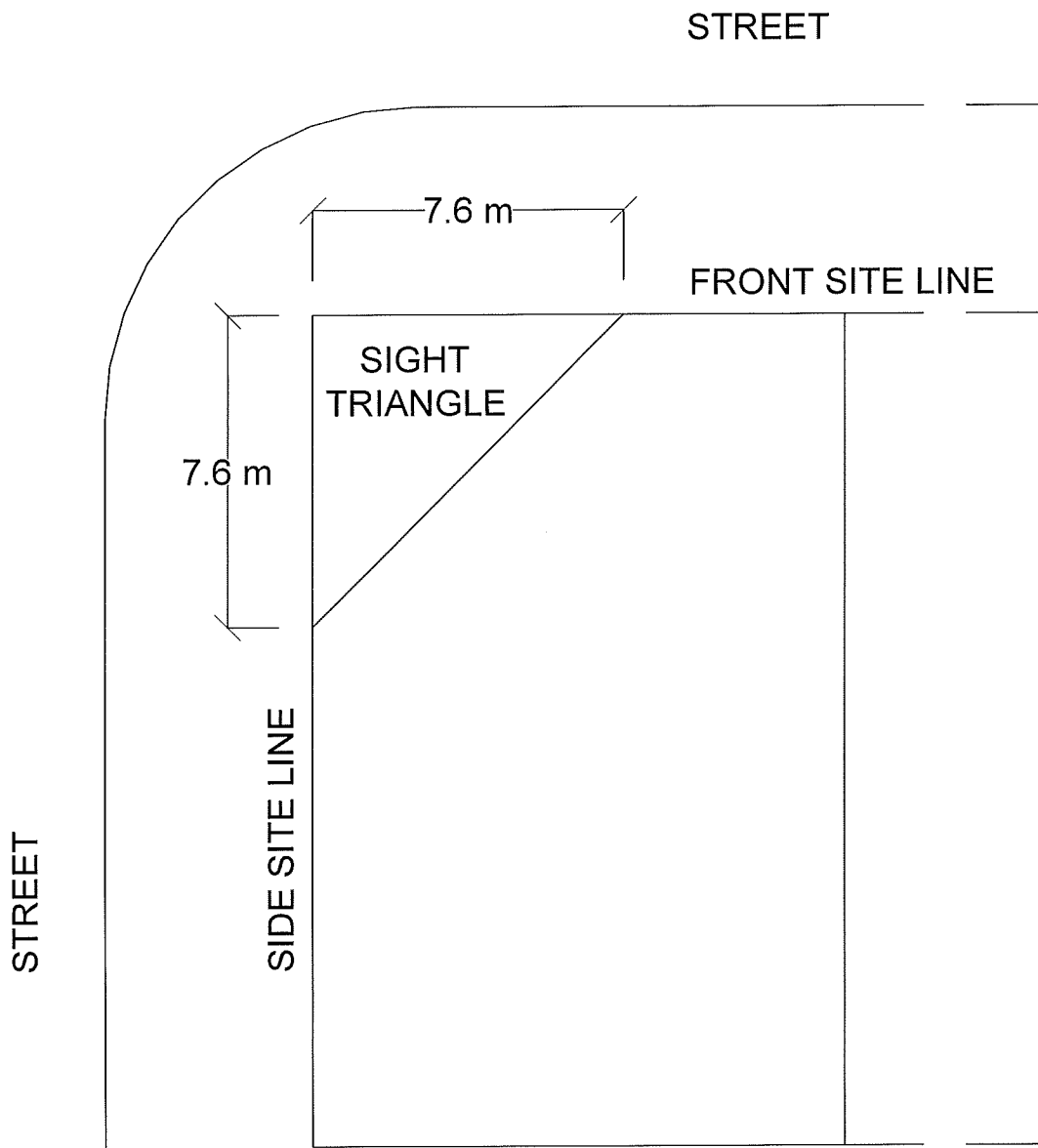
FIGURE 2-3: Sight Triangle
